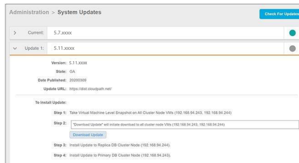
FIGURE 1 System Updates Screen for Upgrading a Cluster from 5.7.4774 (or Later) to 5.12.5514
